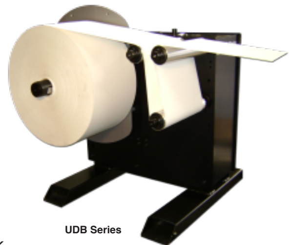
UDB Series with optional electronic web guide and splice table
